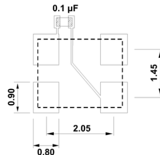
Solder Pad Layout(mm)
