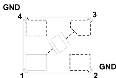
Top View Crystal Connection
