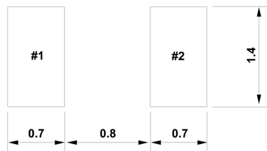
Suggested Layout
