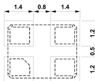
Top View Suggested Layout
