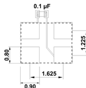
Solder Pad Layout(mm)
