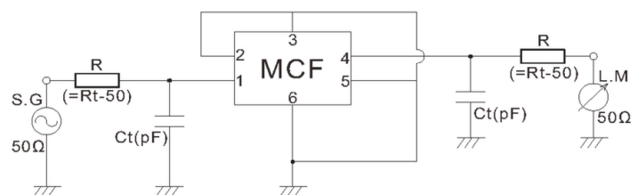
Measurement Circuit
